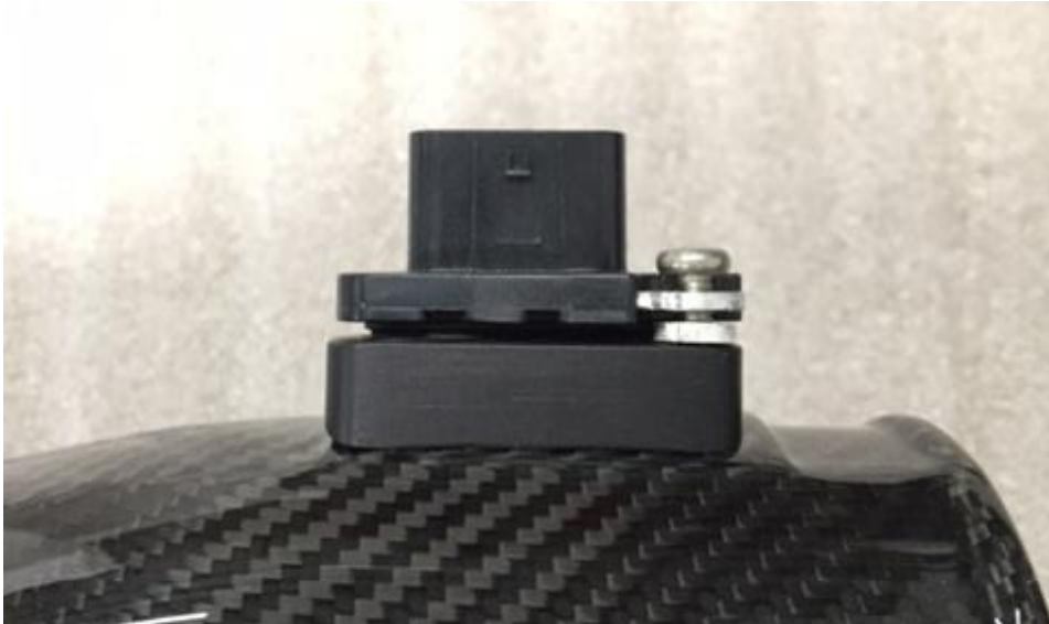
17. With the spacer in place as shown – secure the sensor with the supplied M4 screws.
