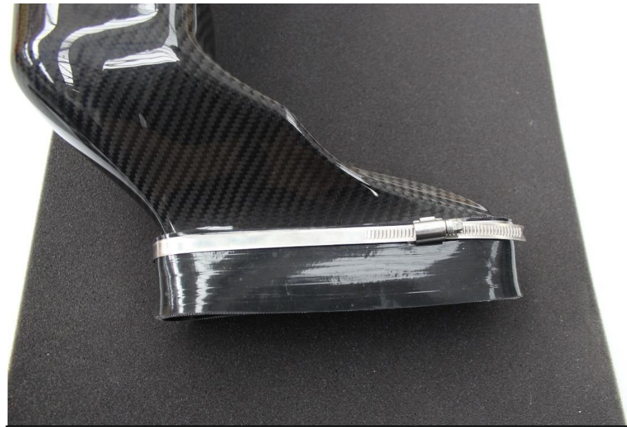
13. Push the silicon hoses onto each airbox and use 1 hose clamp around the carbon as shown. Leave 25mm overhang as shown in next step.
