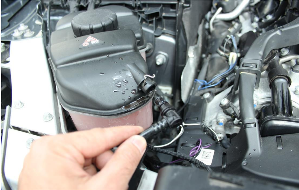
12. Remove the small coolant tube from the top of the coolant tank.
