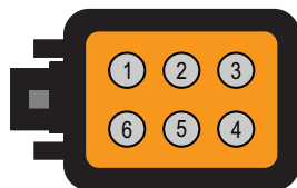
6-pin Auxiliary Connector Wire side view
