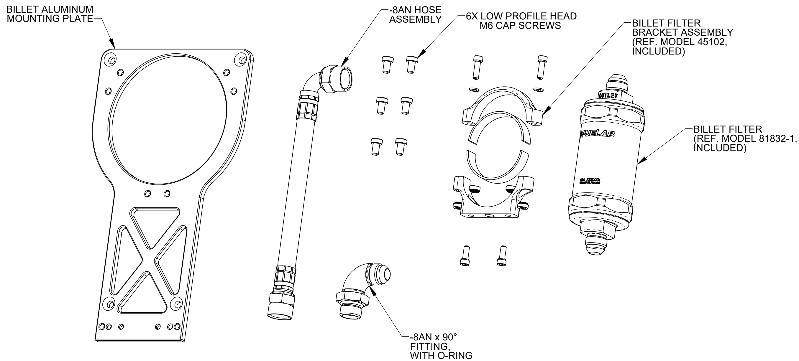
ACCESSORY KIT CONTENTS SHOWN ABOVE
