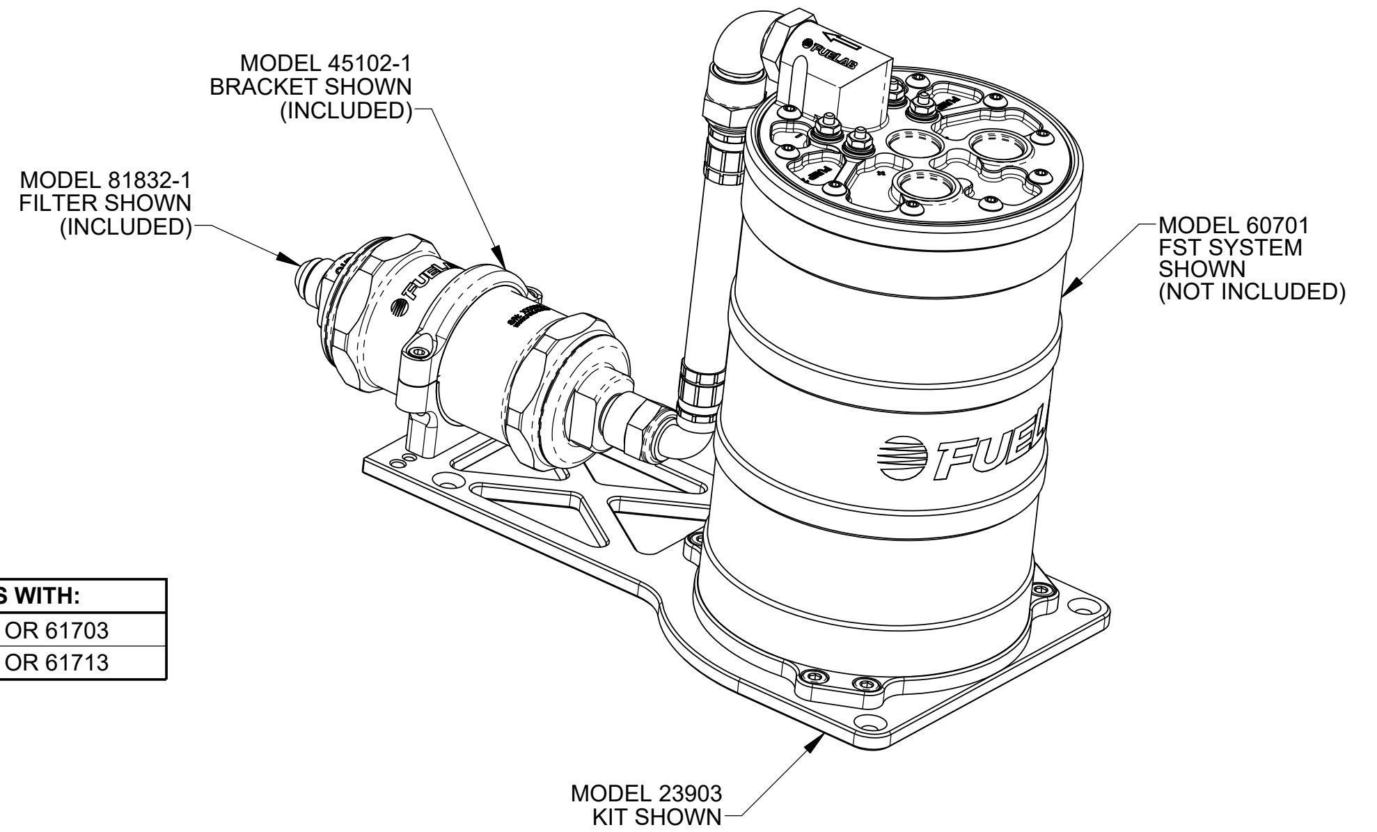
ISOMETRIC VIEW SHOWN (WITH MODEL 60701 SHOWN ASSEMBLED)
